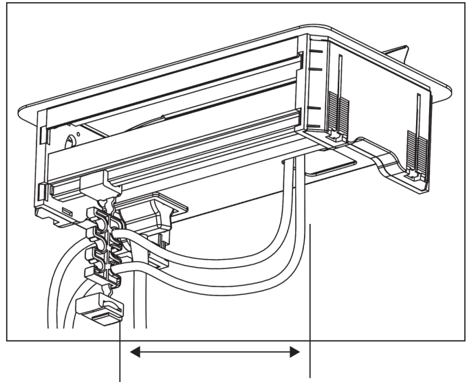
ALLOW SUFFICIENT CABLE SLACK
